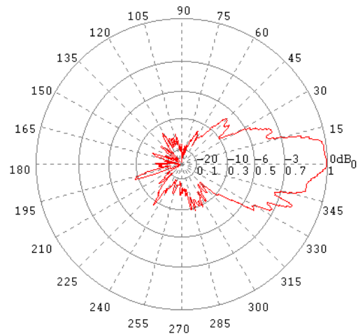
E-Ebene / E-Plane 16 GHz
