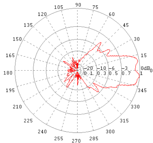
E-Ebene / E-Plane 11 GHz
