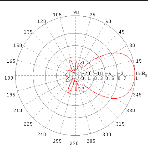
H-Ebene / H-Plane 2 GHz
