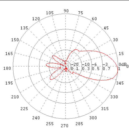
E-Ebene / E-Plane 2 GHz
