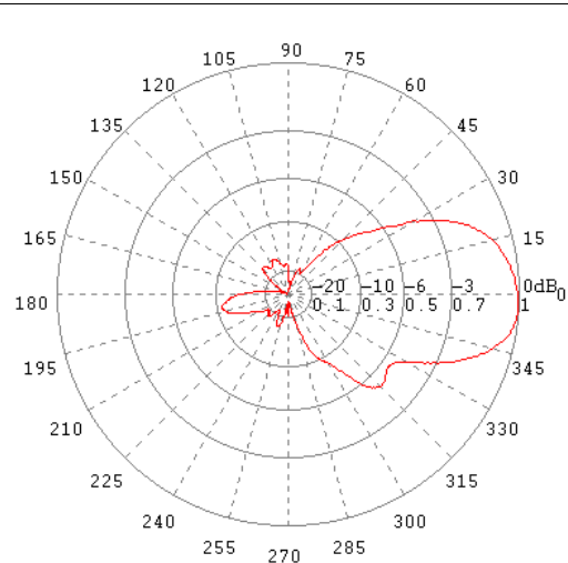
E-Ebene / E-Plane 3 GHz
