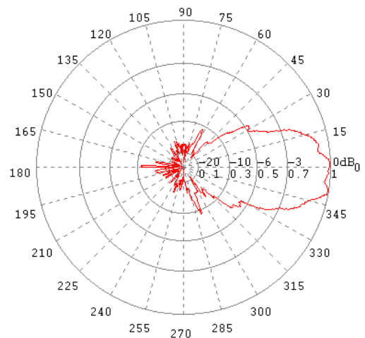
H-Ebene / H-Plane 12 GHz
