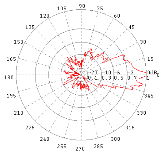
E-Ebene / E-Plane 17 GHz
