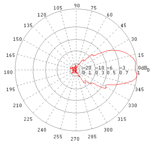
E-Ebene / E-Plane 8 GHz
