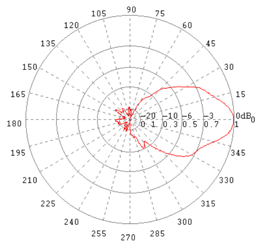
E-Ebene / E-Plane 5 GHz
