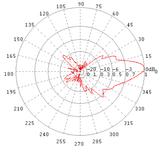
E-Ebene / E-Plane 7 GHz
