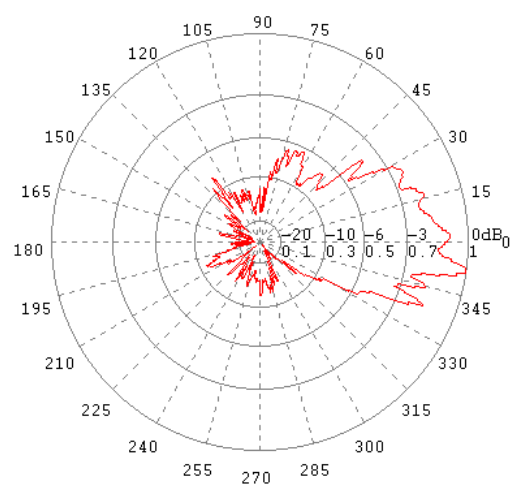
E-Ebene / E-Plane 18 GHz
