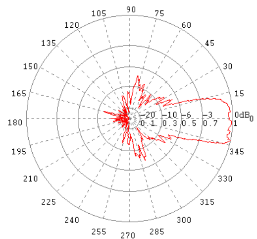
H-Ebene / H-Plane 17 GHz
