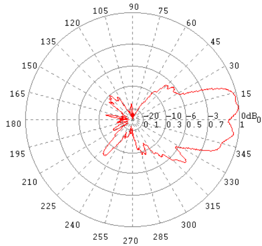
E-Ebene / E-Plane 10 GHz
