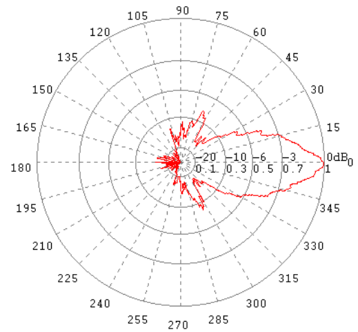
H-Ebene / H-Plane 16 GHz
