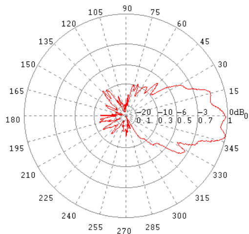
E-Ebene / E-Plane 12 GHz
