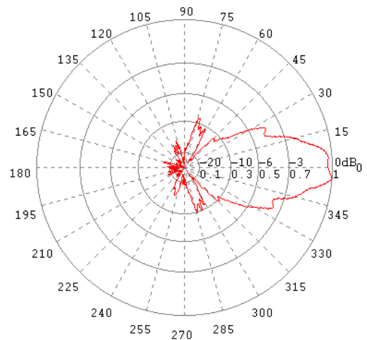
H-Ebene / H-Plane 11 GHz
