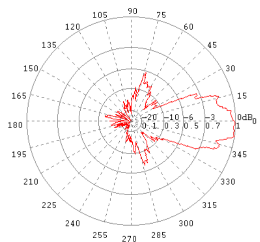
H-Ebene / H-Plane 18 GHz
