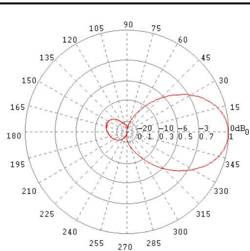
E-Ebene / E-Plane 1 GHz
