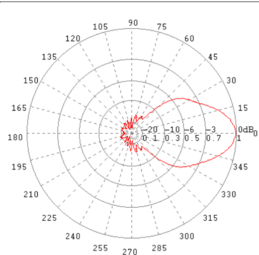
H-Ebene / H-Plane 3 GHz
